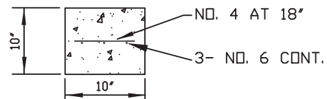
FOOTING DETAIL
