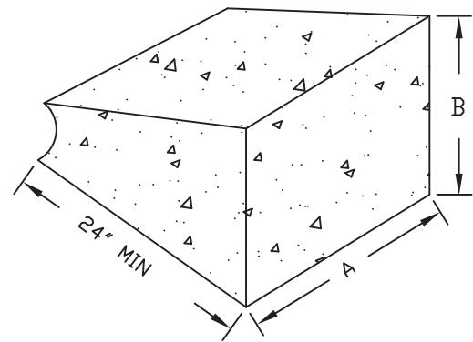
THRUST BLOCK
